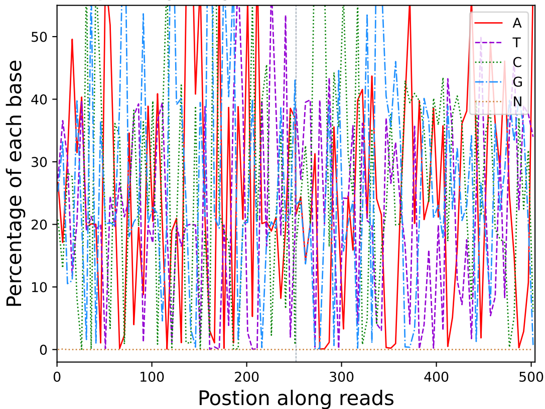
Base percentage along reads (R10719)
